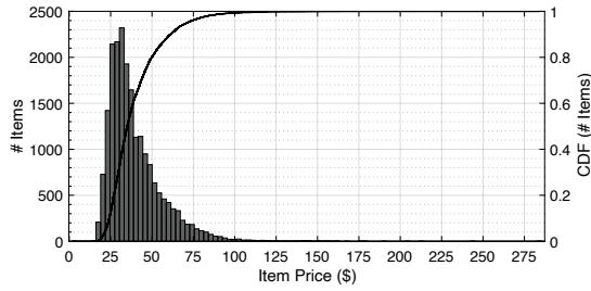
Fig. 4: Item listing prices in Amazon MX vs. the number of items (with the CDF plot).
