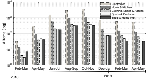
Fig. 5: # of items for the most popular five categories grouped by item addition date in the gap item records.
