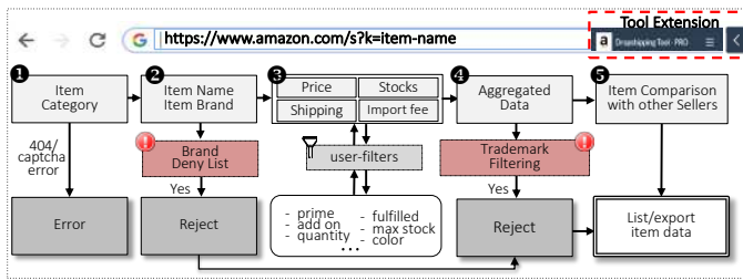
Fig. 8: Reverse engineered execution flow of malicious dropshipping tool ( Software-Mal ), a subscription-based product research & listing tool designed for abusive dropshippers.
