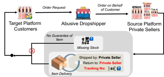
Fig. 9: Fulfillment process used in abusive dropshipping.
