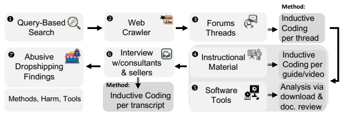
Fig. 2: Abusive dropshipping data collection process.
